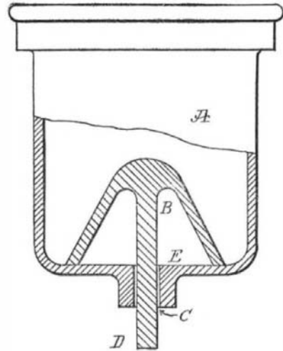
AUTOMATIC LUBRICATING CUP.
