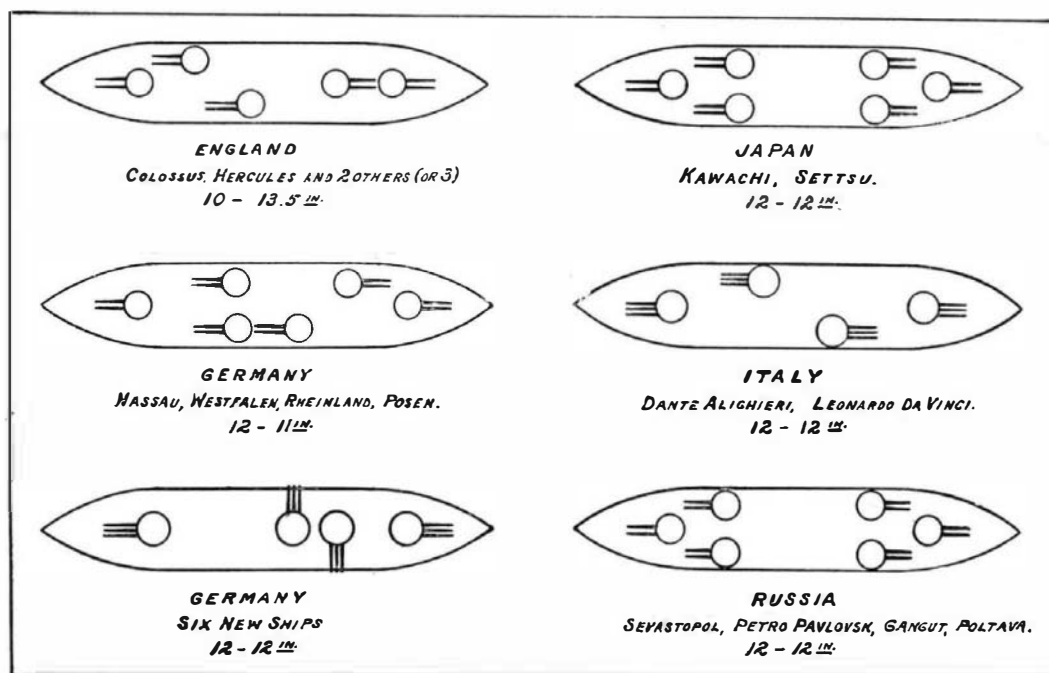
LATEST "DREADNOUGHT" DESIGNS OF THE NAVAL POWERS.
