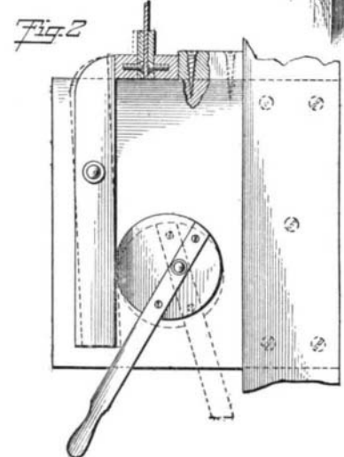
A HOME-MADE SAW VISE.
