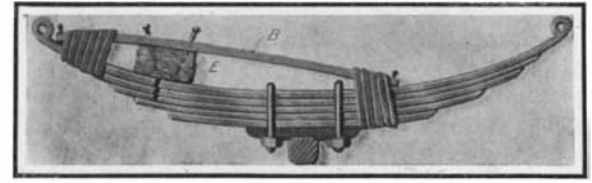
Fig. 2.—REPAIRING A BREAK AT ONE END OF THE SPRING.
