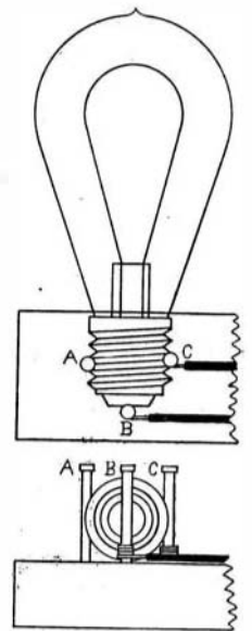
A SIMPLE LAMP RECEPTACLE.
