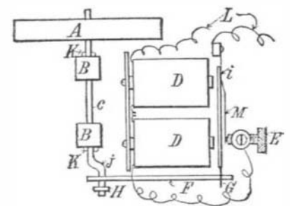
A SIMPLE ELECTRIC ENGINE.
