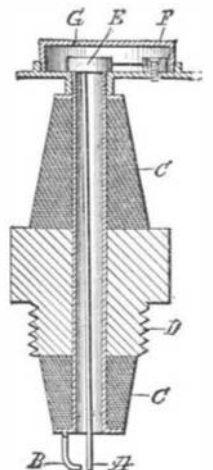
THE HANDY MAN'S SPARK PLUG.
