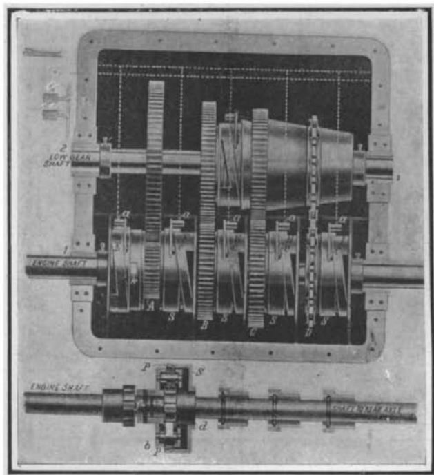
A NOVEL SPEED-CHANGING GEAR.
