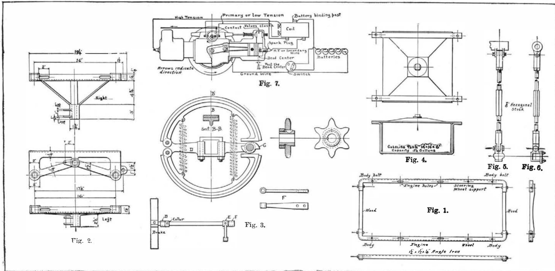
DETAILS OF MOTOR BUGGY PARTS.
