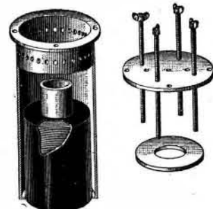
Reduced Fac-simile, Simple Impregnating Chamber.
