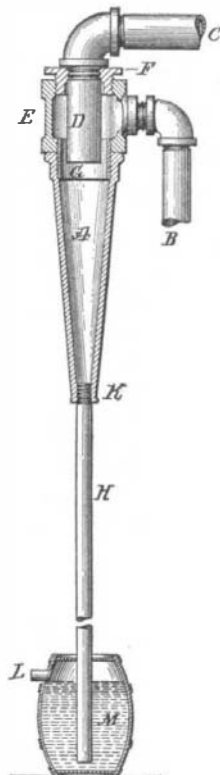
THE HOME-MADE VACUUM CLEANER.
