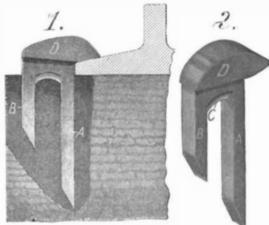
RAILROAD SPIKE.
