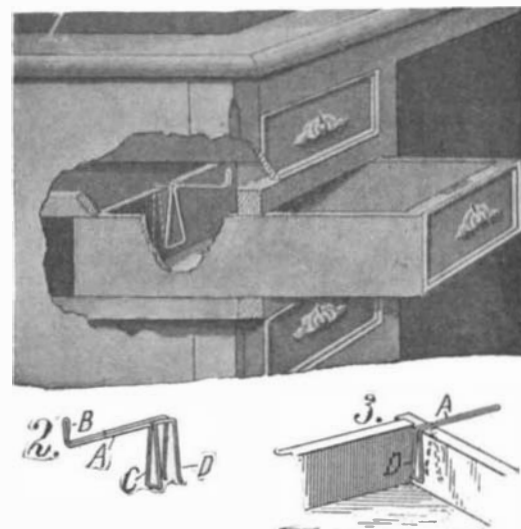
A SIMPLE DRAWER STOP.
