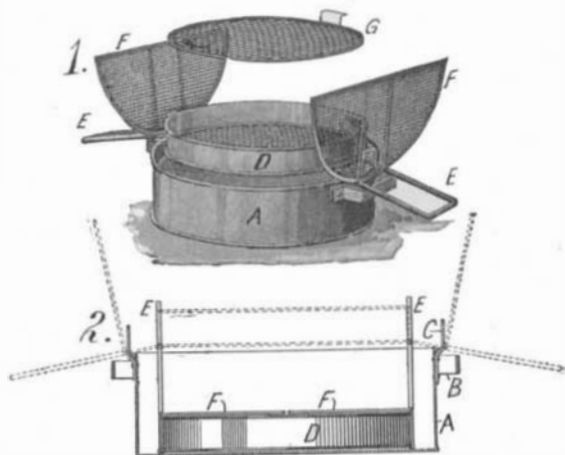
FRYING DEVICE.
