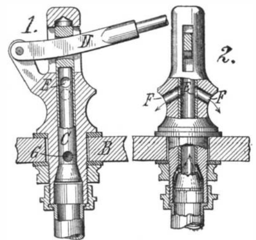
VALVE FOR FLUSH TANKS.
